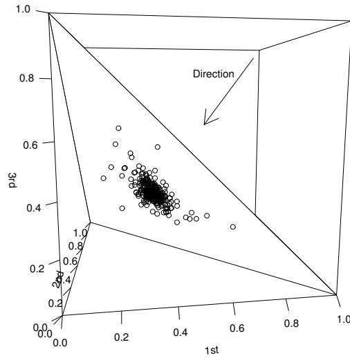
Figure 1: 3-dimensional case.
